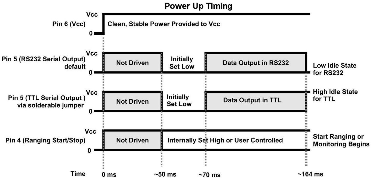
RS232/TTL solderable jumper (and if used, external temperature sensor) connected before powering.
